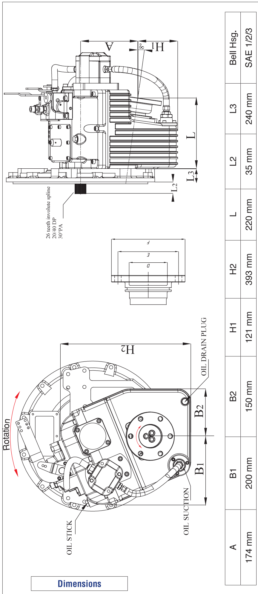
SAE Flange Dimensions
